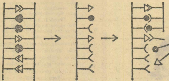
Schema moleculei ADN
